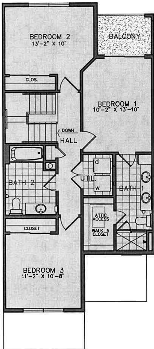
TYPE C 2 UPPER PLAN C1.5 SCALE: 1/8" = 1'-0" 0 2' 4' 6'
